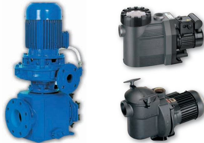
Figure 4: Circulating pump for solar circuits. Cast iron housing, chrome nickel steel shaft, cast iron or gunmetal impeller (source : Herborner Pumpentechnik)
