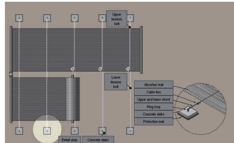
Figure 10: Fixing of absorbers with tension belts and concrete slabs on a flat surface
