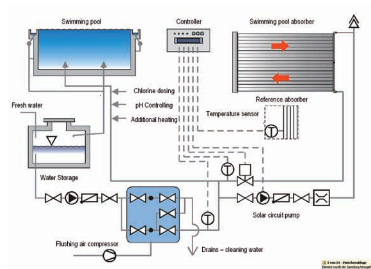
Figure 7: Circuit diagram of a large absorber system with additional solar pumps
