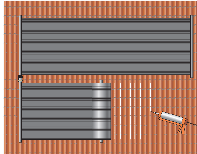
Figure 12: Bonding of absorbers on a pitched tiled roof
